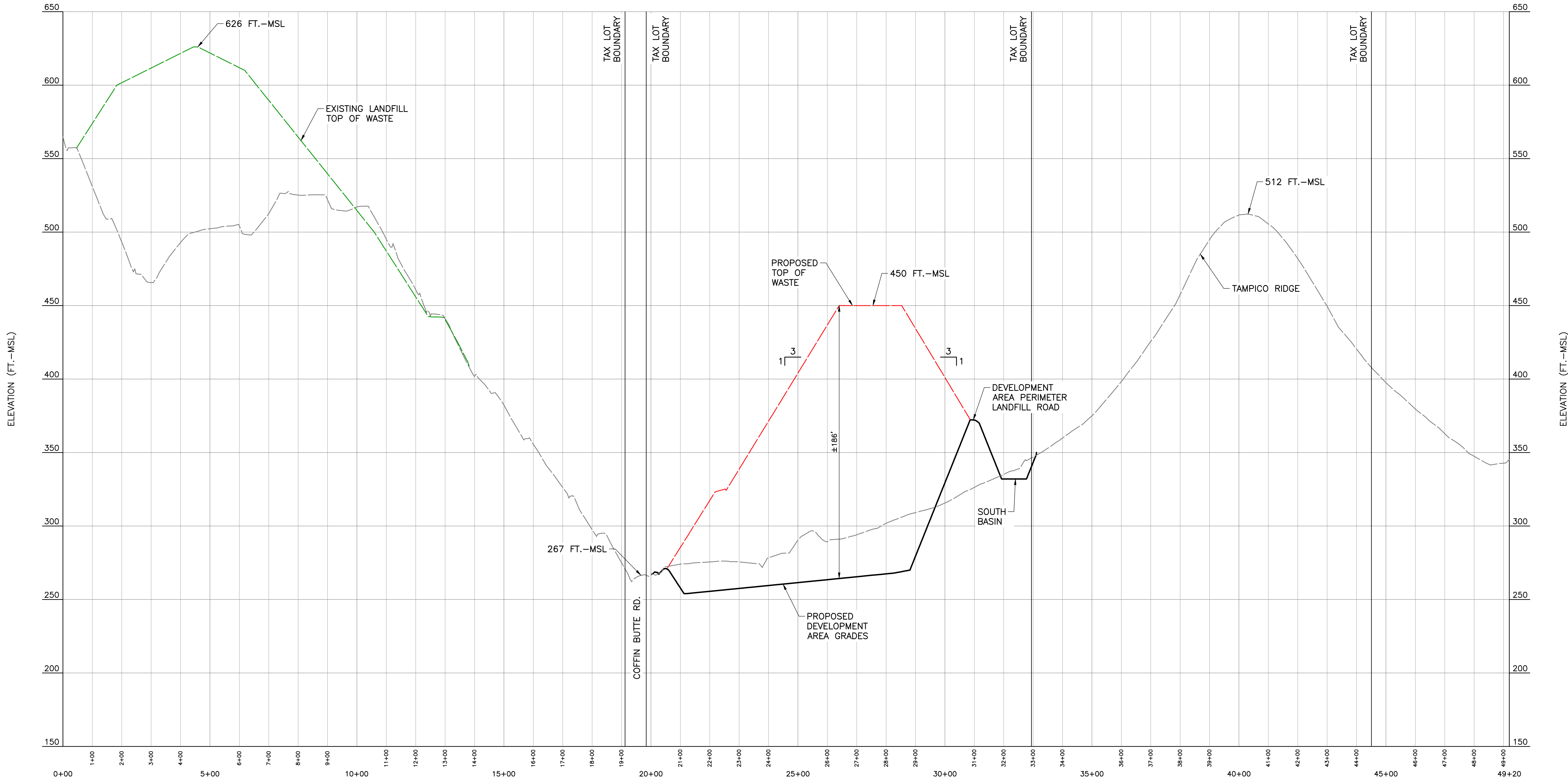
CROSS SECTION K3 - K3 SCALE H:1"=200'; V:1"=40'
